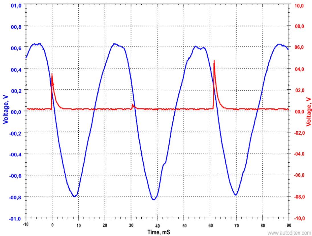
Fig.9. Exhaust pulses and 1 st cylinder sync signal, 1997 Opel Astra F 1.8 16V, DIS ignition
