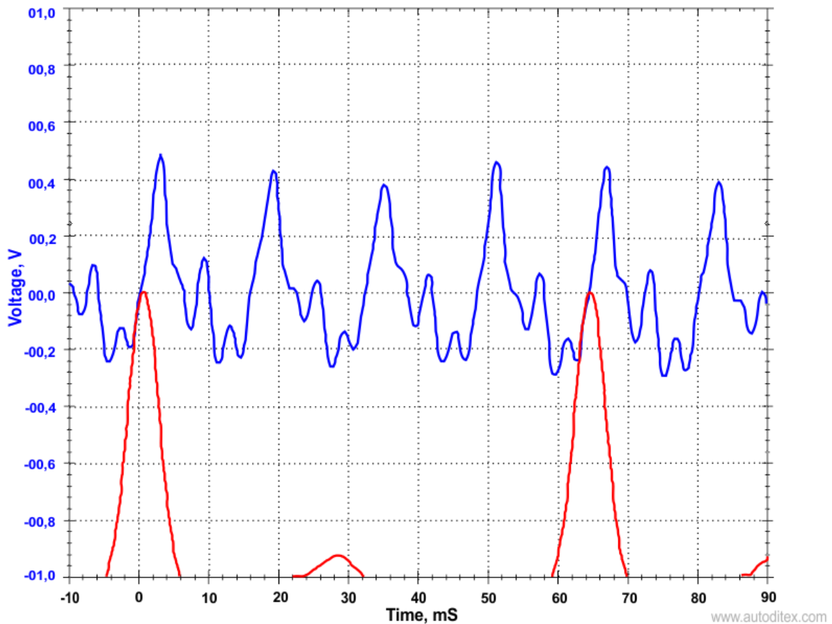
Fig.5. Pressure Pulse Sensor intake manifold and Cylinder pressure sensor
