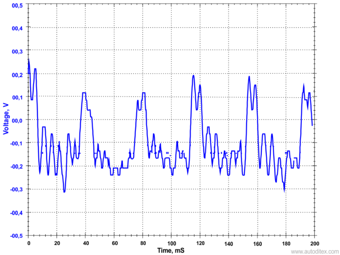
Fig.8. Exhaust pulses on 2009 Toyota Auris 1.4 VVT-I
