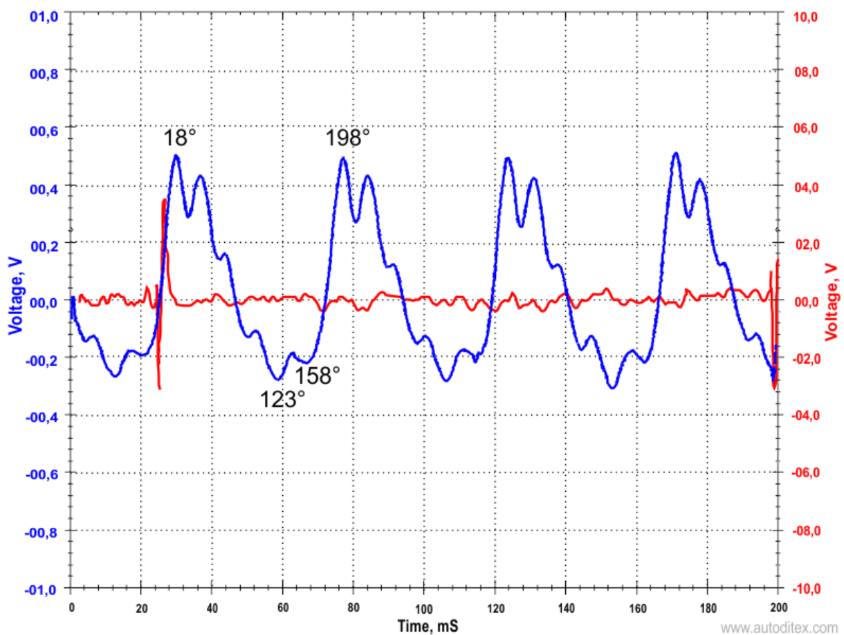
Fig.3. Pressure Pulse Sensor intake manifold pulses and the first cylinder sync signal.
