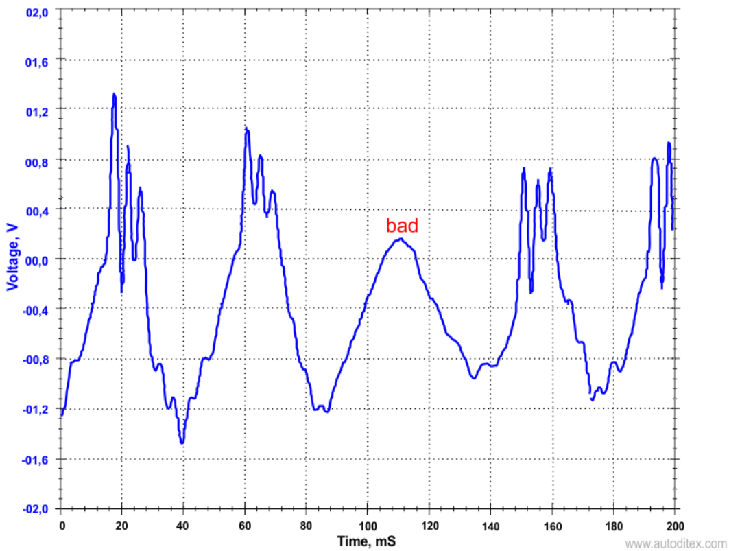
Fig.11. Bad injector on Honda Accord 2, PPS is connected to the fuel pressure regulator
