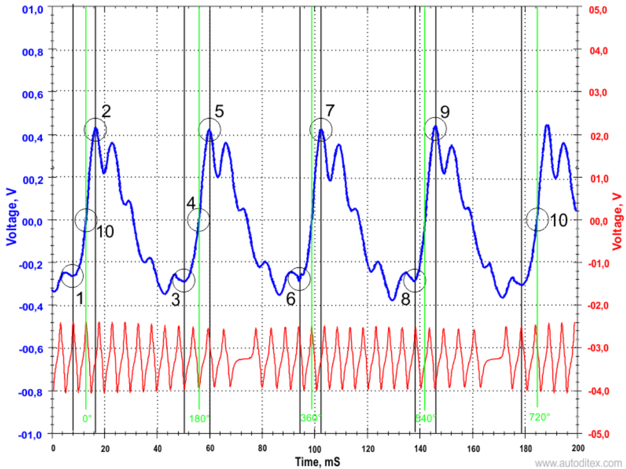
Fig.4. Pressure Pulse Sensor intake manifold pulses and the crankshaft signal
