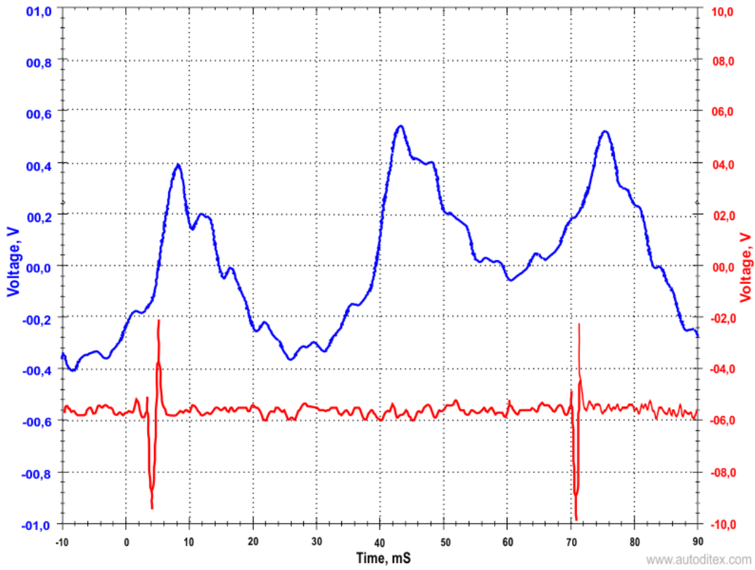
Fig.10. Graphic shows a burned valve (PPS is connected to the intake manifold)
