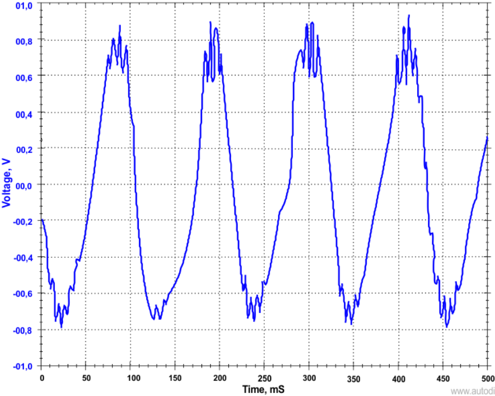
Fig.7. Intake manifold pulsation signal Toyota Rav4. Engine is cranking (engine not started)
