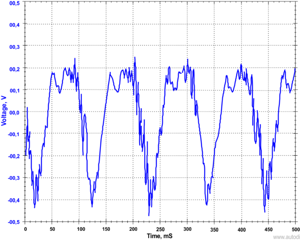
Fig.6. Exhaust gases pulsation signal Toyota Rav4. Engine is cranking (engine not started)
